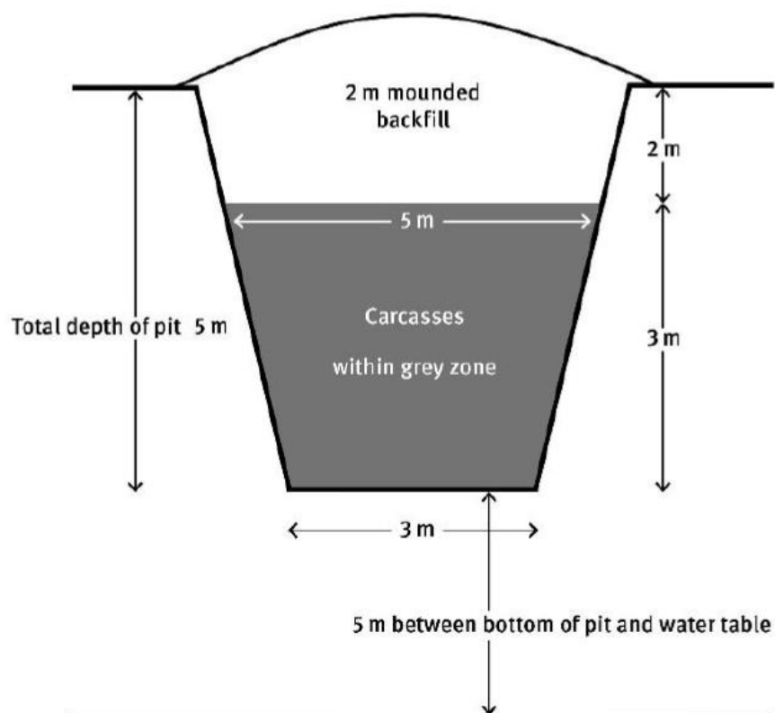
Figure 2 – Traditional battered burial pit
